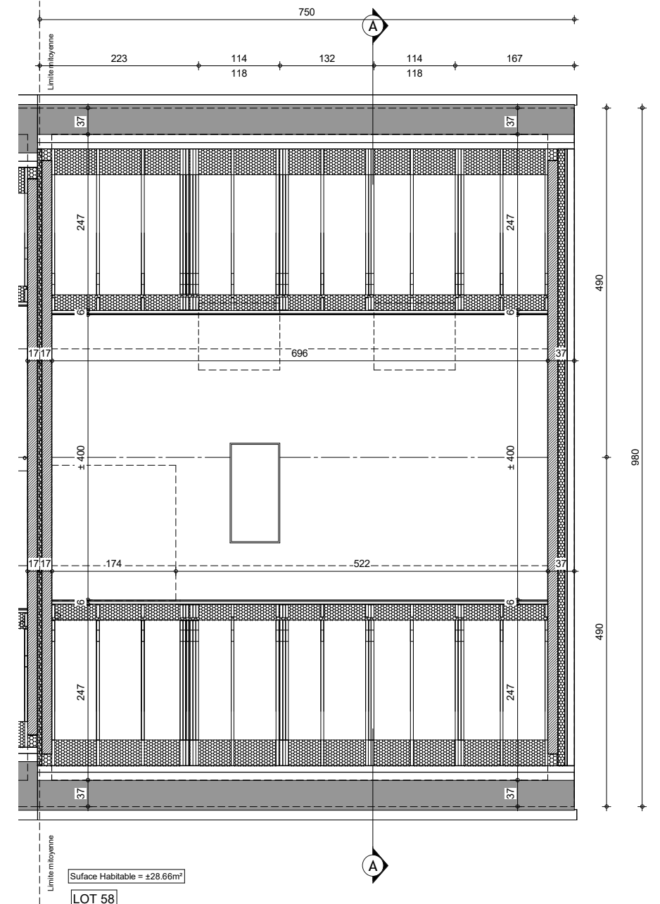
COMBLE AMENAGABLE
